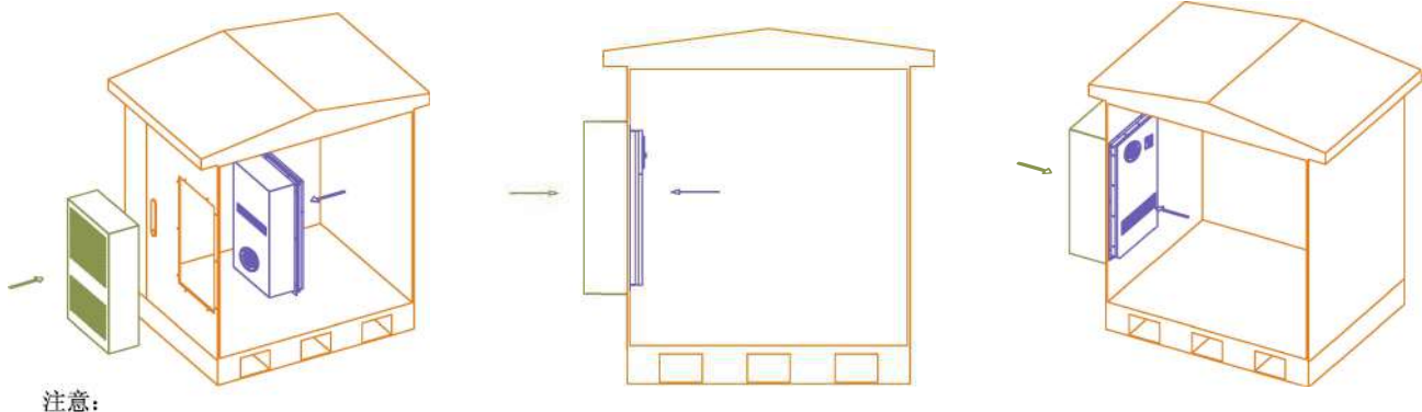
Figure 3-Installation Instruction
