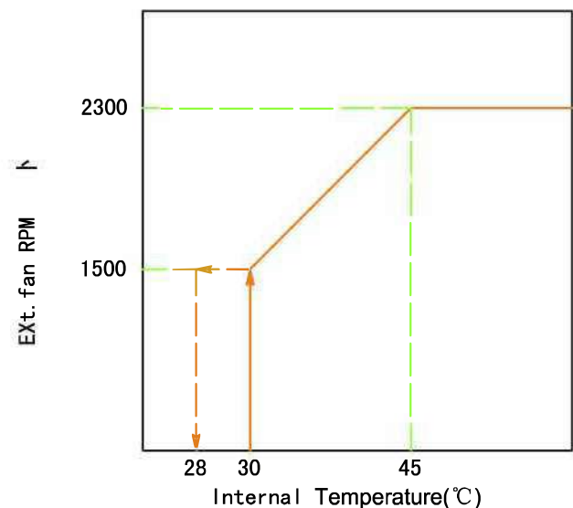
Ext.Fan Speedvs. Cabinet inside temperature Curve
